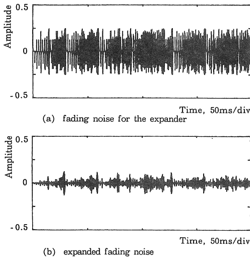
Fig.3 Noise reduction effect over silent duration.
